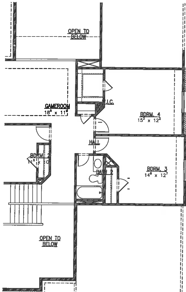
UPPER FLOOR
