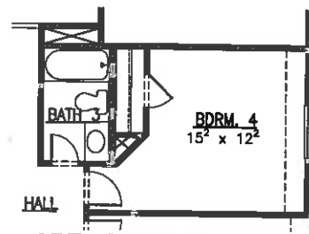
OPT. BATH 3
